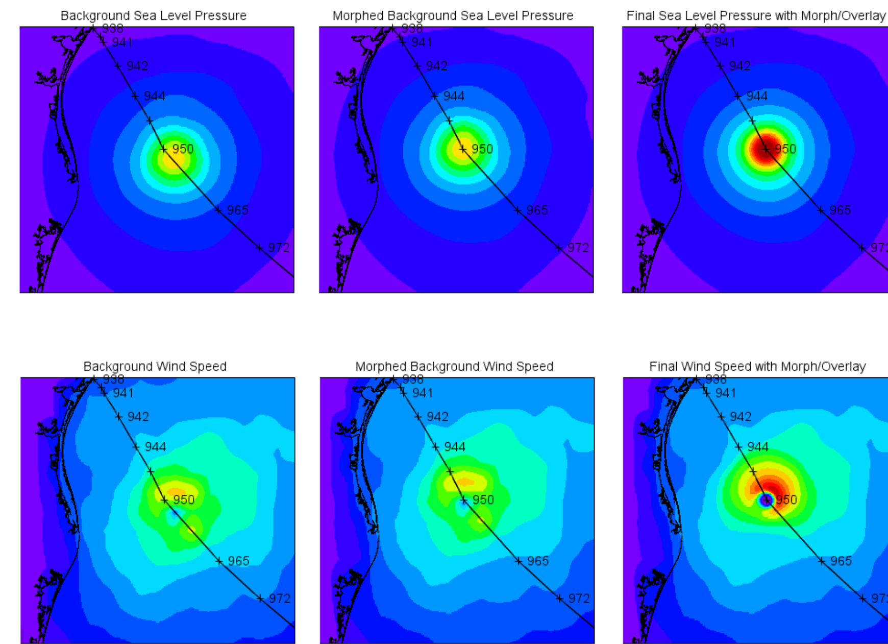
Figure 5. Contours of Sea Level Pressure (mb, top) and wind speed (knots, 30-minute average, bottom) for ECMWF analysis (left), repositioned ECMWF analysis morphed to Harvey location (middle) and final analysis including morphed ECMWF and overlay of tropical cyclone model output (right)
