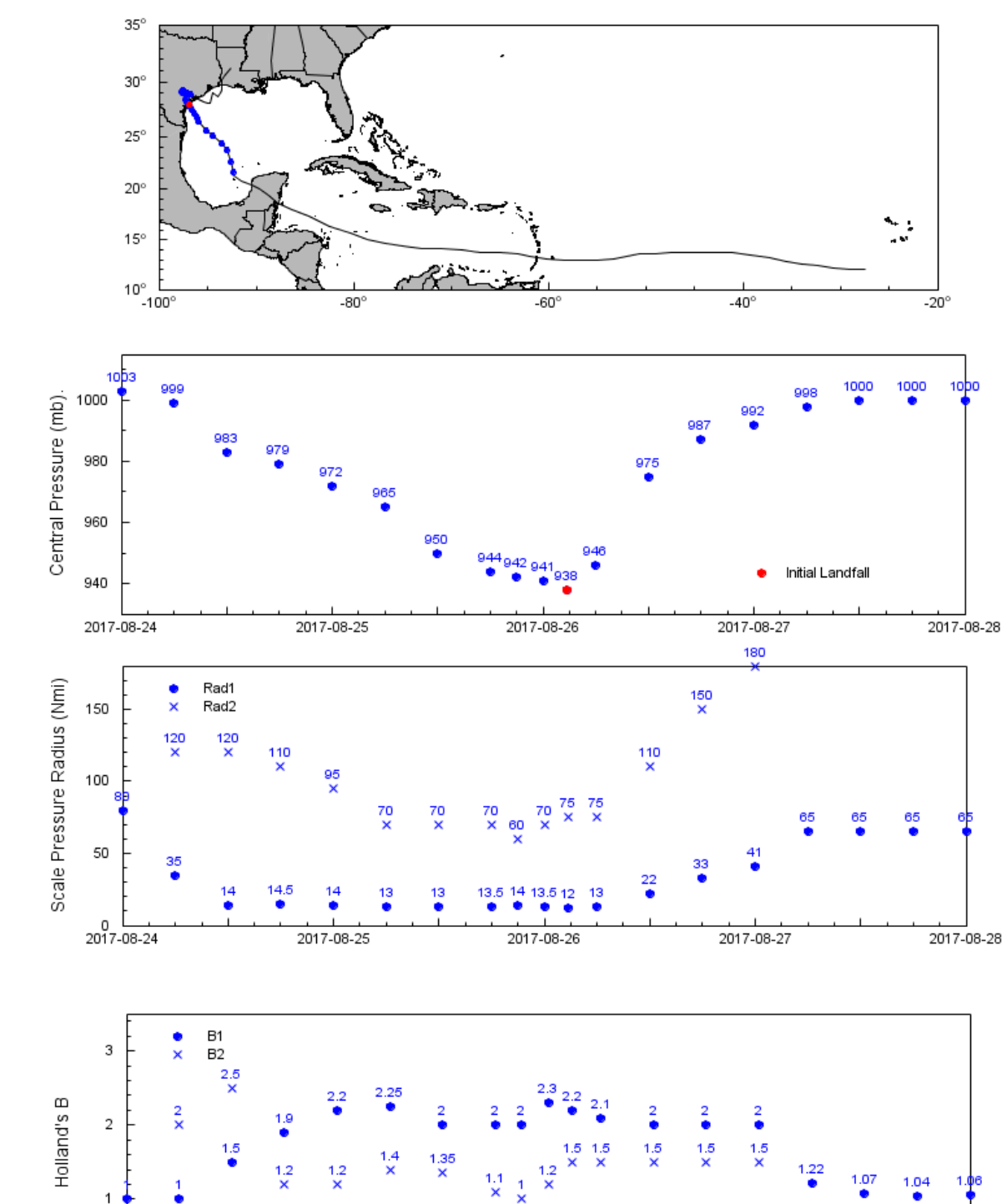
Figure 2. Track (top) and TropPBL inputs of sea level pressure (mb), scale pressure radius (Nmi) and B during Harvey from Aug 24-28 2017
