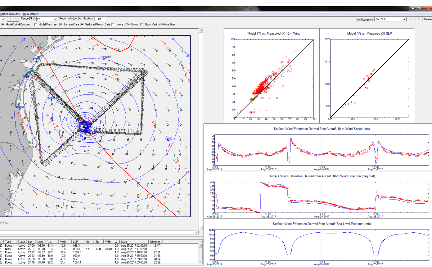
Figure 4. Time series comparison of aircraft stepped frequency microwave radiometer surface winds and TropPBL winds (kts, 30-minute average)
